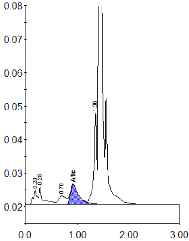
Peak table - ID: 10530259
